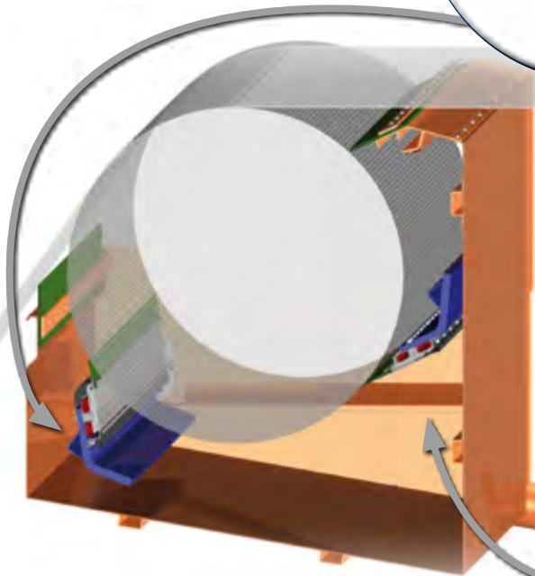
Save-all with integrated doctors for couch rolls
